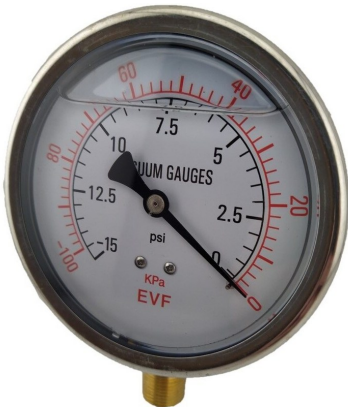
LIQUID FILLED VACUUM GAUGE 63MM DIAL
